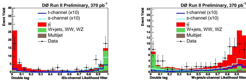
FIGURE 6. Data to Monte Carlo comparison of the discriminant distributions for combined e+jets and \mu +jets channels in the double-tagged sample in the s -channel single top search. Comparison for the tb/t\bar{t} filter (left) and for the tb/W +jets filter (right).
