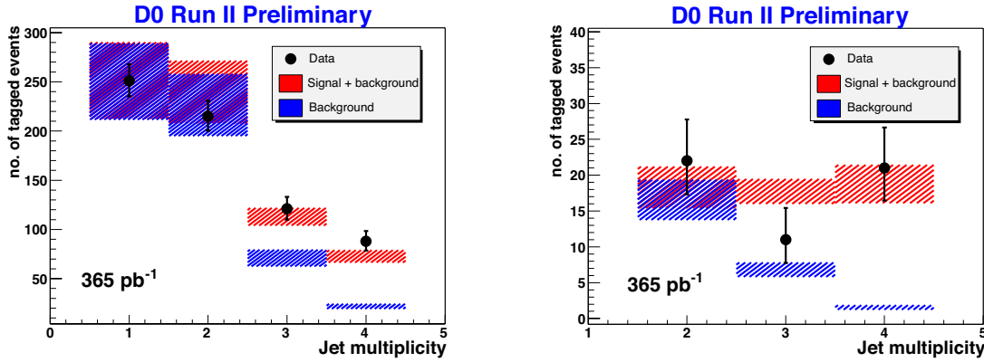
FIGURE 4. Measurement of the t\bar{t} production cross section in the lepton+jets final state using 365 \text{ pb}^{-1} of D\bar{O} data. Left: Jet multiplicity distribution of data (points) compared to Standard Model backgrounds and top for events having a single b -tagged jet (left) and those having both b quark jets tagged (right).
