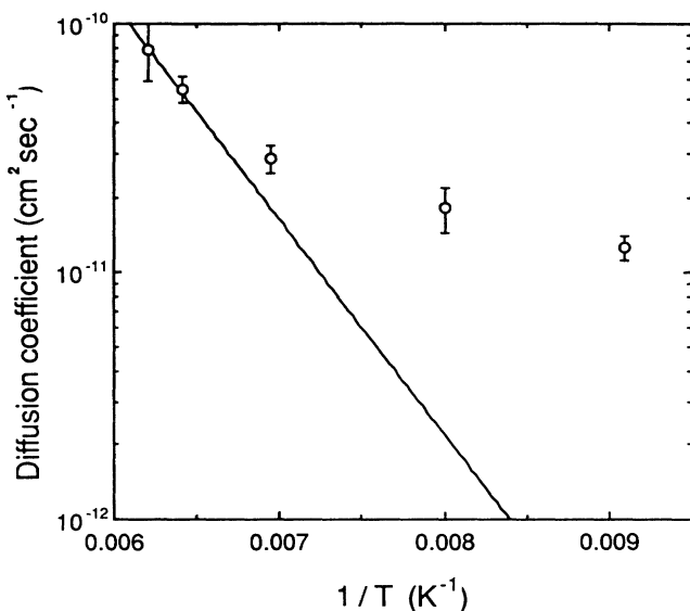
FIG. 3. Arrhenius plot of the diffusion coefficient D(T) = \alpha(T)a^2/2\pi^2 . The solid line passes the first two data points. The slope yields an activation energy E_{\text{diff}} = 3.5 kcal/mol.
